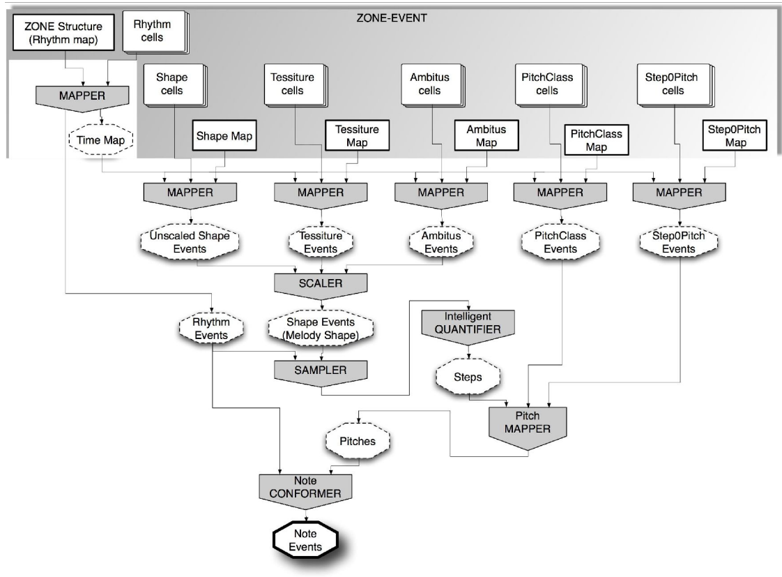
Figure. 5. Melody Generation Algorithm
